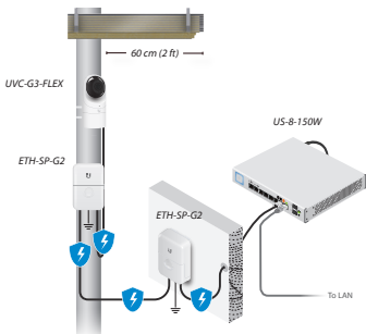
Diagram Showing Use of Ethernet Surge Protectors
