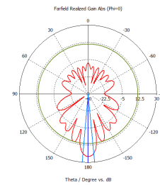
Vertical Polarization PHI 0
