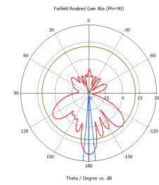
Horizontal Polarization PHI 90
