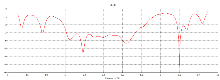
Vertical Polarization Return Loss
