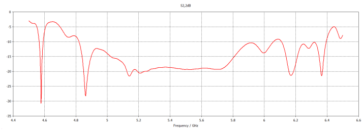
Horizontal Polarization Return Loss
