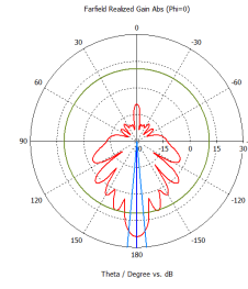
Horizontal Polarization PHI 0
