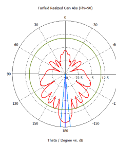
Vertical Polarization PHI 90
