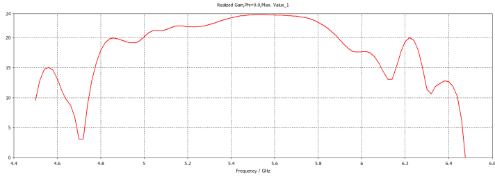
Horizontal Polarization Gain
