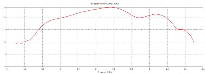
Vertical Polarization Gain
